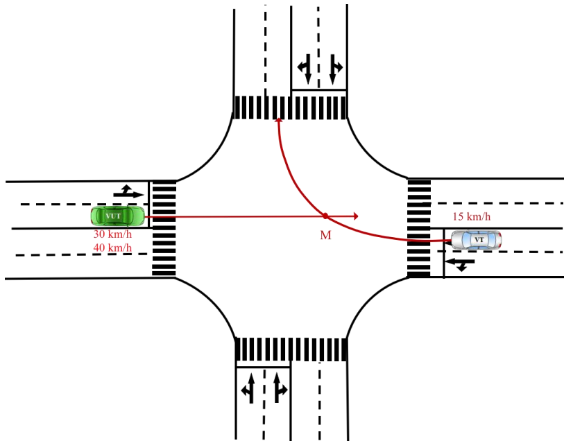
Figure 20 VUT travelling straight with an oncoming passenger car turning right
