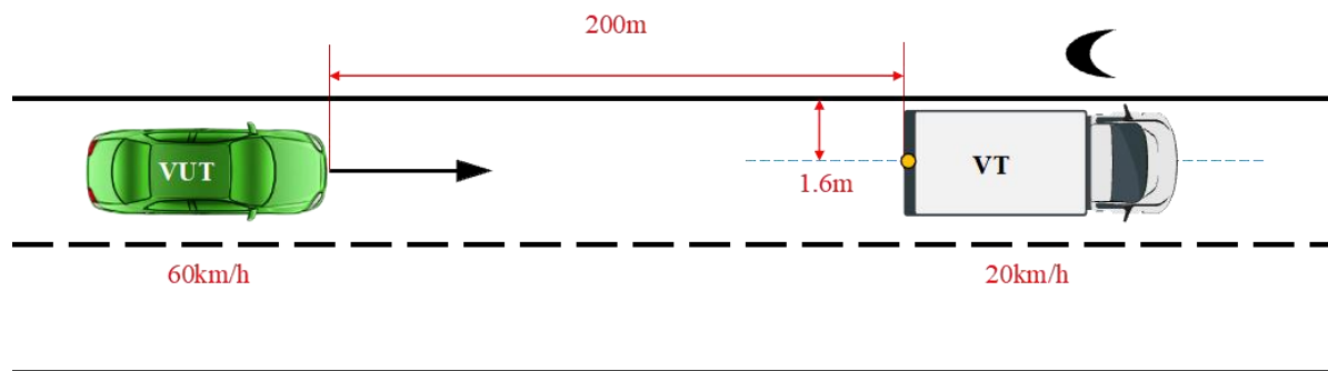
Figure 16 Moving light truck ahead
