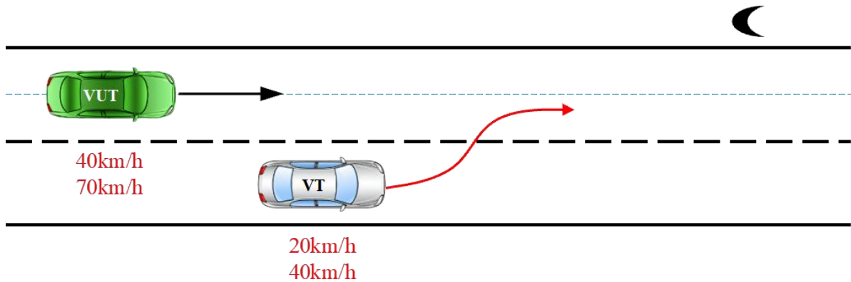
Figure 17 Passenger car cutting in at night
