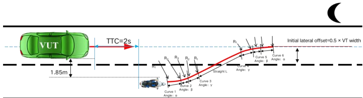
Figure 25 Target cut-in path
