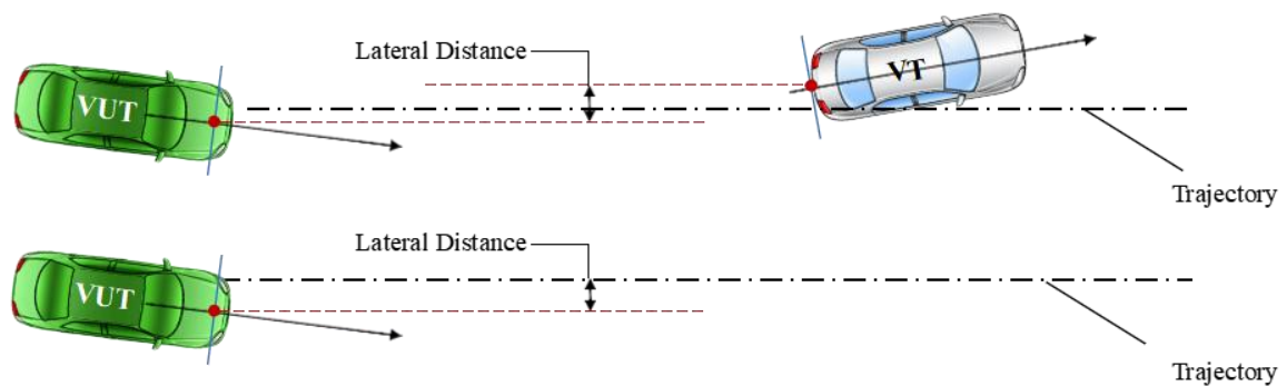
Figure 1 Lateral offset
