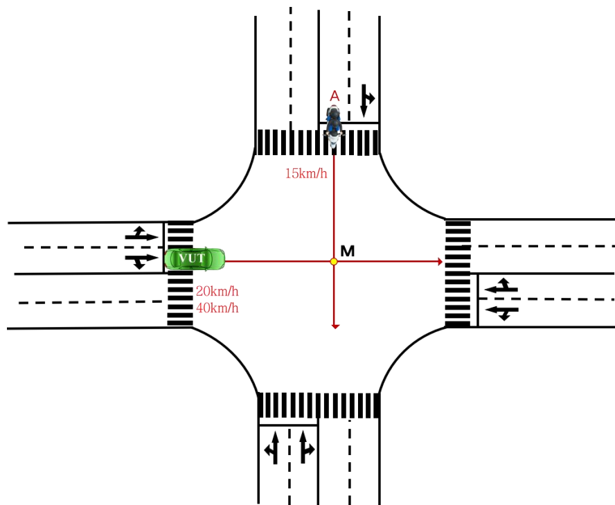
Figure 26 Motorcycle carrying a child crossing ahead
