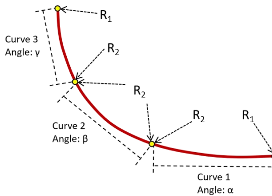
Figure 21 VT right-turn path
