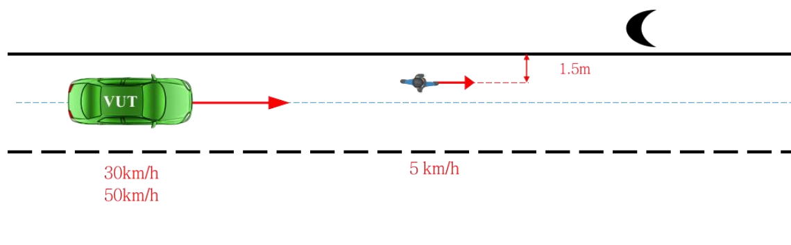
Figure 29 Pedestrian walking longitudinally at night
