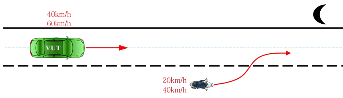
Figure 24 Motorcycle carrying a child cutting in ahead at night
