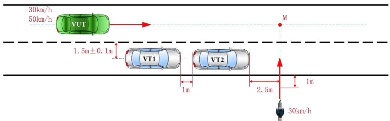
Figure 27 Obstructed motorcycle crossing ahead
